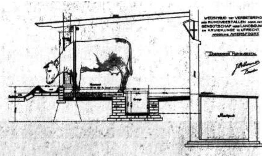
Ontwerp grupstal, architect Pothoven, Leusden, 1913
